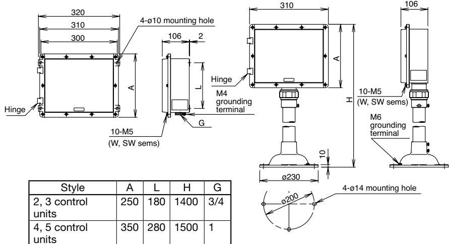
Control Unit Mounting Hole
