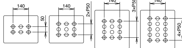
Control Unit Mounting Hole
